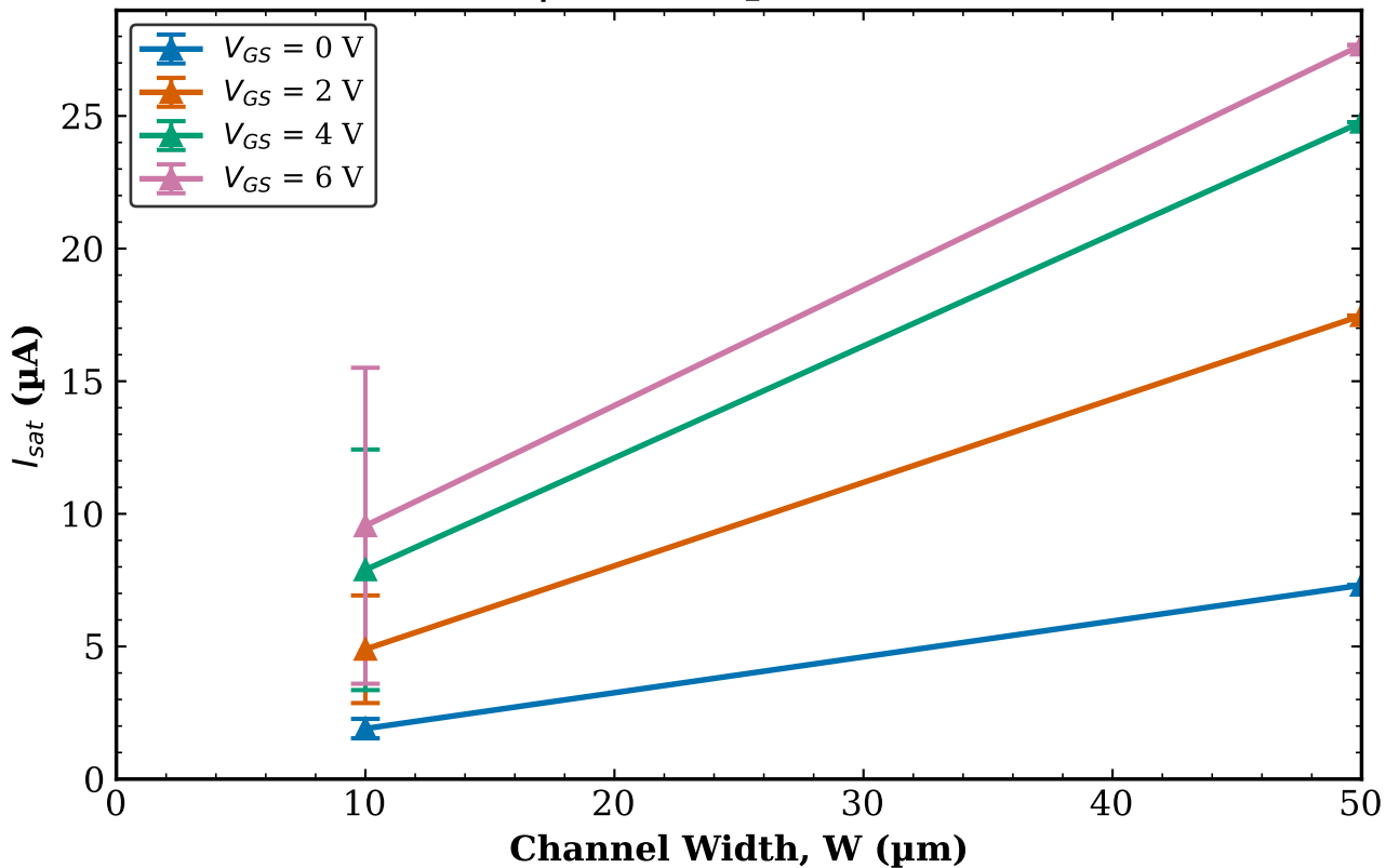
TFT2 Combined (Tr. 1 & 2) I_{sat} vs W | L = 20\text{ }\mu\text{m} (mean \pm std)
